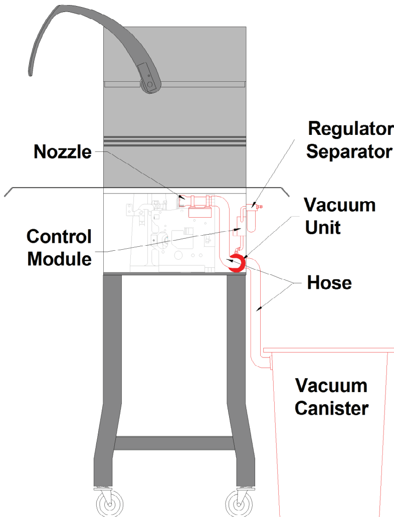
VTR parts kit (includes canister)
